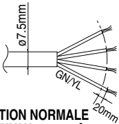
SECTION NORMALE DU TUYAU 0.75mm² H07RN-F
